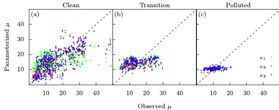
Figure 6. Scatterplots of observed versus parameterized shape parameter ( \mu ) using the relationships specified in Table 2 for each aerosol regime: clean ( N_a < 900 \text{ cm}^{-3} , flights M1, RA1 and RA2), transition ( N_a \sim 2500 \text{ cm}^{-3} , flight AD1), and polluted ( N_a > 3000 \text{ cm}^{-3} , flights AD2 and AD3).
