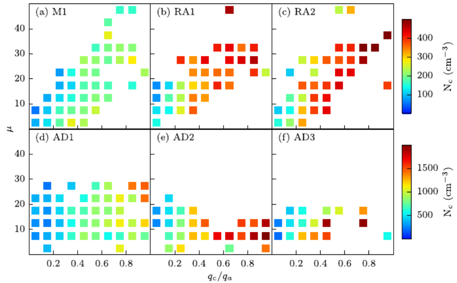
Figure 5. Averages of the cloud droplet number concentration ( N_c ) for intervals of five units of \mu and 0.1 units of q_c/q_a in the observations.
